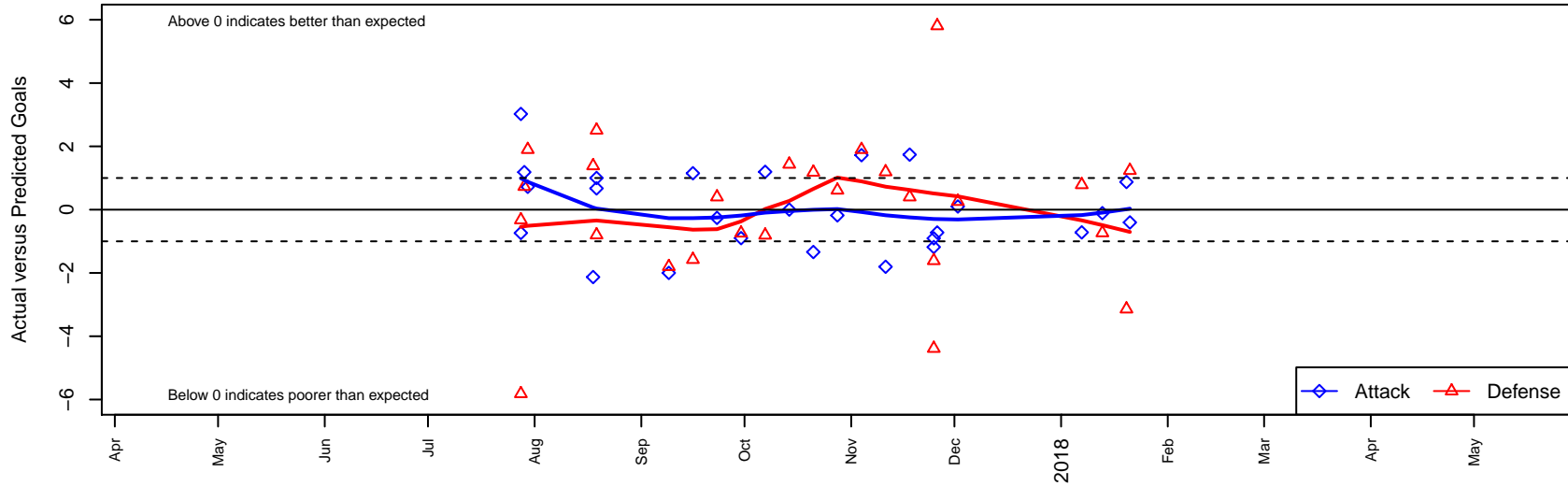
NSC Chaos B04 Dots are actual minus expected GF (blue circles) and GA (red triangles). Blue line is smoothed change in attack strength. Red is smoothed change in defense strength.
